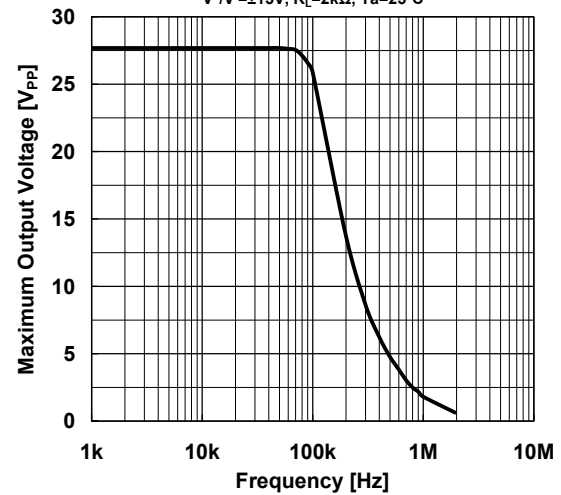
Maximum Output Voltage vs. Frequency V^+/V^-=\pm 15V , R_L=2k\Omega , T_a=25^\circ C
