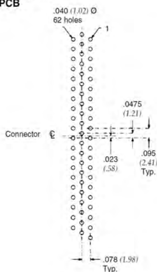
62 High-Density Pin/PCB
