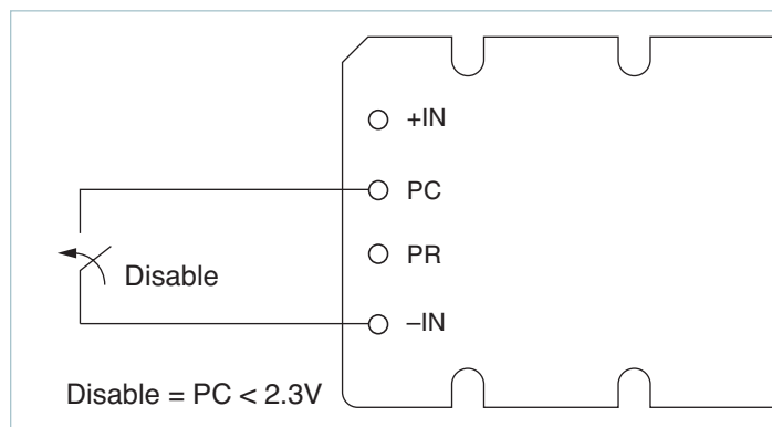
Figure 2 — Module enable/disable
