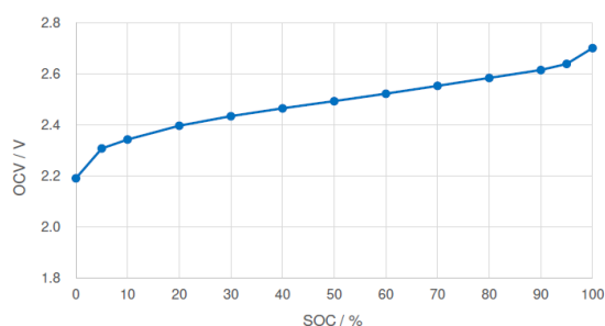
Figure 11 - SoC OCV curve (SLB03090LR80*)
