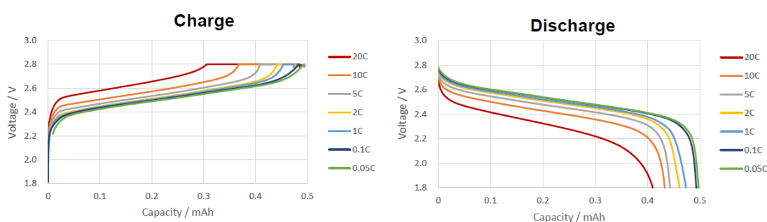
Figure 9- SLB charge/discharge characteristics (SLB03070LR35*)
