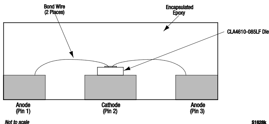
Figure 5. Cross-Sectional View of the CLA4610-085LF
