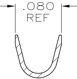
INSULATION RANGE .061 MAX SECTION G-G
