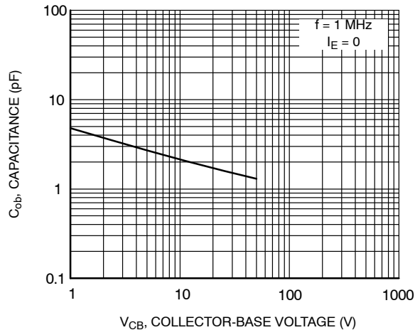
Figure 5. Output Capacitance
