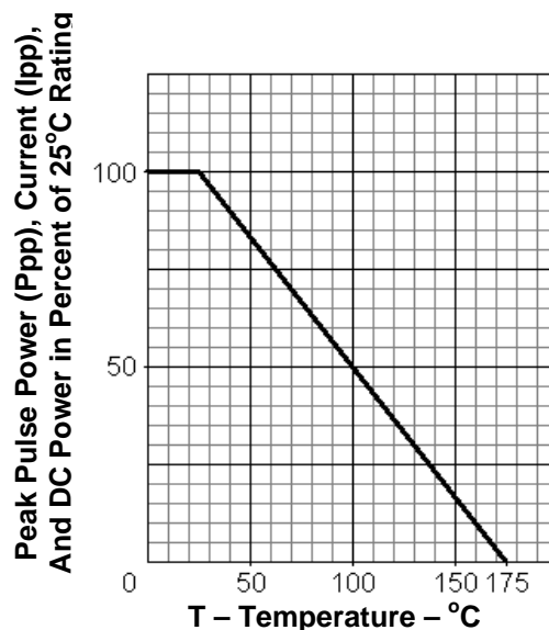
FIGURE 4 DERATING CURVE
