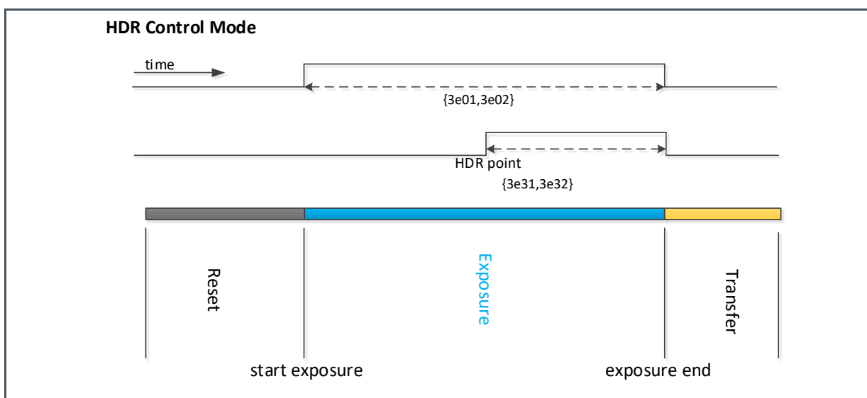
Figure 42: HDR Mode Timing
