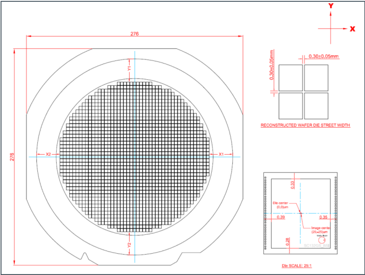
Figure 9: Wafer Dimensions
