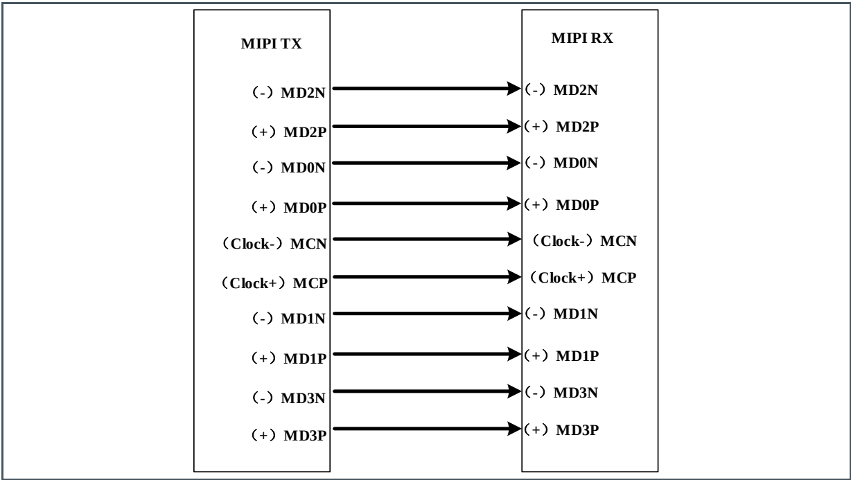
Figure 28: MIPI Interface
