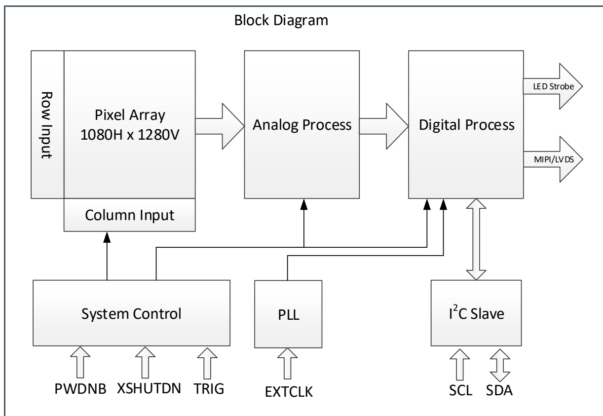
Figure 2: Functional Blocks of Mira130
