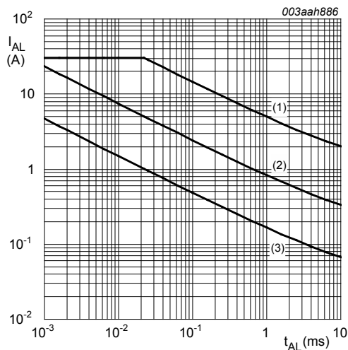
Fig. 4. Avalanche rating; avalanche current as a function of avalanche time (1) T_{j(init)} = 25^{\circ}C ; (2) T_{j(init)} = 150^{\circ}C ; (3) Repetitive Avalanche
