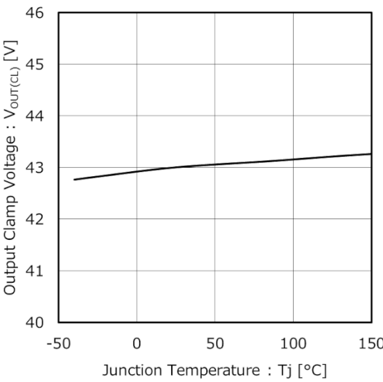
Figure 9. Output Clamp Voltage vs Junction Temperature (IOUT = 1 mA)
