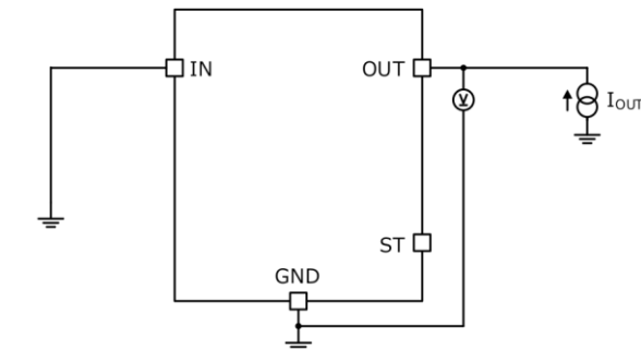
Measurement Circuit for Figure 8 and Figure 9
