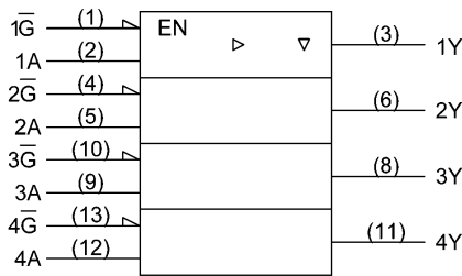
74VHCT125AFT
