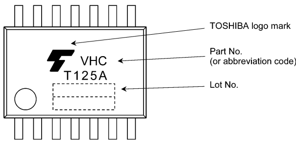
74VHCT125AFT
