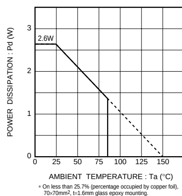
Fig.4 Power dissipation
