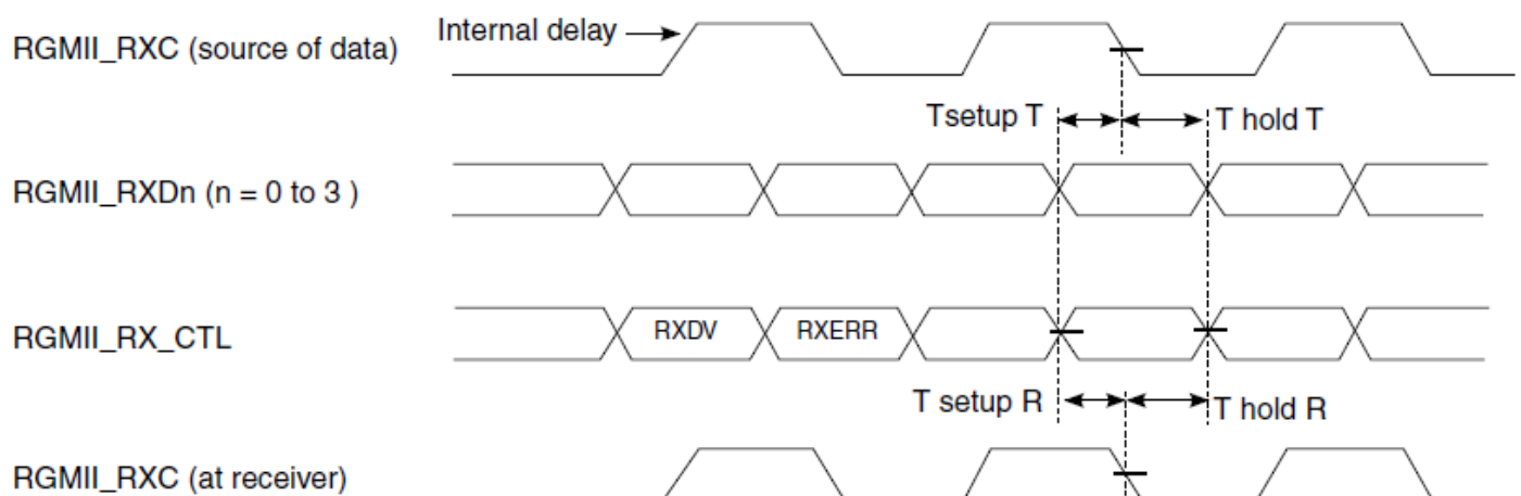
Figure 8. RGMII receive signal timing diagram with internal delay
