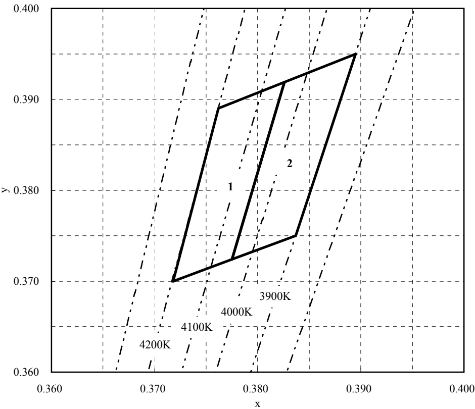
Chromaticity Diagram
