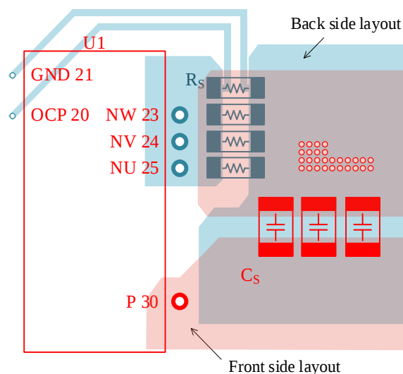
Figure 14-2. Peripheral Layout Example of C_S (Double-sided Board)
