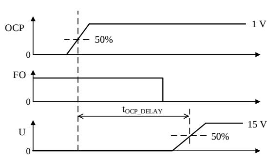
Figure 4-2. OCP Pin Detection Delay Time Definition
