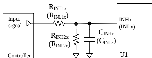
Figure 13-6. Filter Circuit for INHx or INLx Pin
