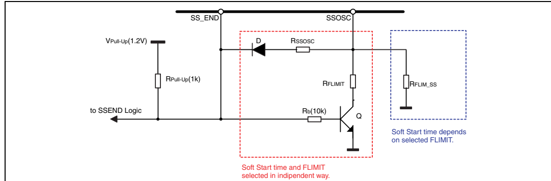
Figure 19. SSOSC connection
