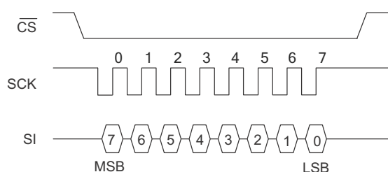
Figure 5. SPI Mode 3
