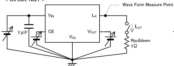
< Circuit No.7 >
