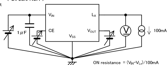
< Circuit No.4 >
