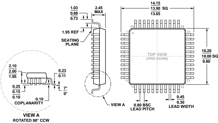
COMPLIANT TO JEDEC STANDARDS MO-112-AA-2 Figure 1. 44-Lead Metric Quad Flat Package [MQFP] (S-44-2) Dimensions shown in millimeters
