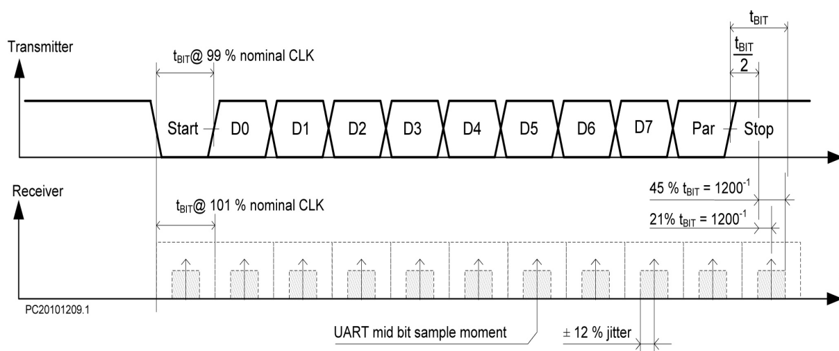
Figure 9. Clock Skew
