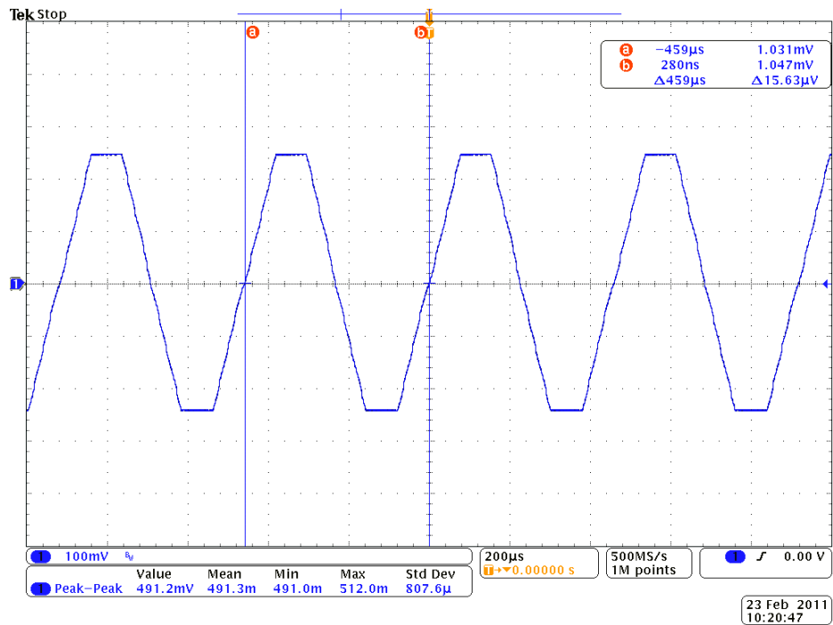
Figure 11. Output Waveform (Space)
