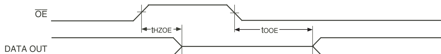
Figure 9. Output Enable Timing, IDT72403 and IDT72404 Only
