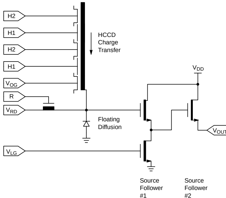
Figure 4. Output Architecture
