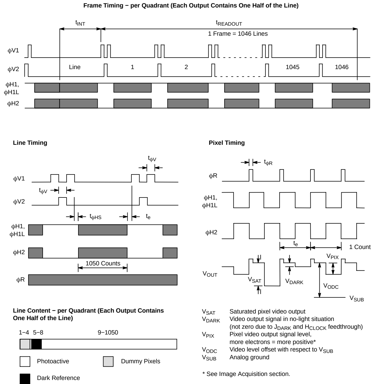
Figure 17. Timing Diagrams
