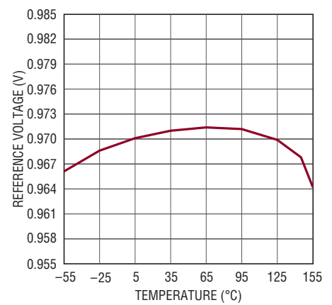
Reference Voltage
