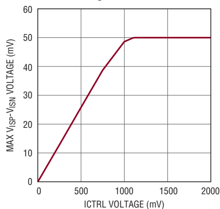
ICTRL Voltage
