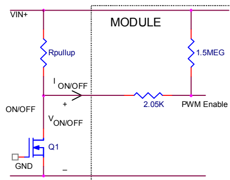
Circuit configuration for using positive On/Off logic
