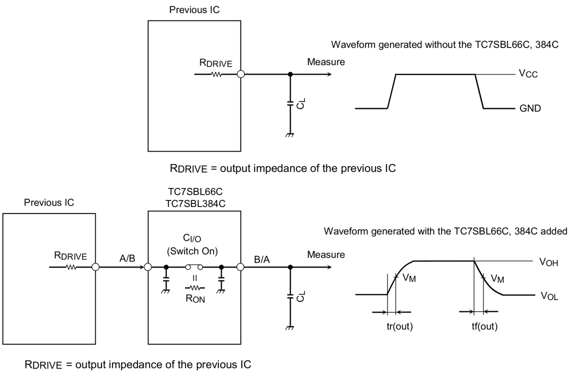
Fig. 12.1 Calculation Circuit
