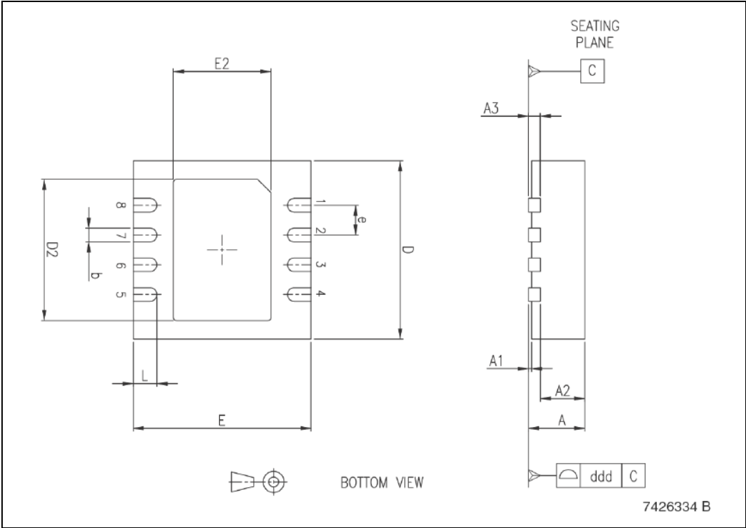
Figure 34. Package dimensions
