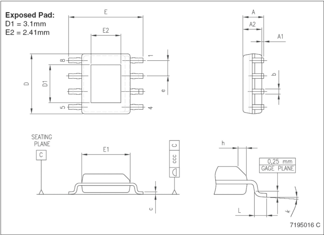
Figure 35. Package dimensions
