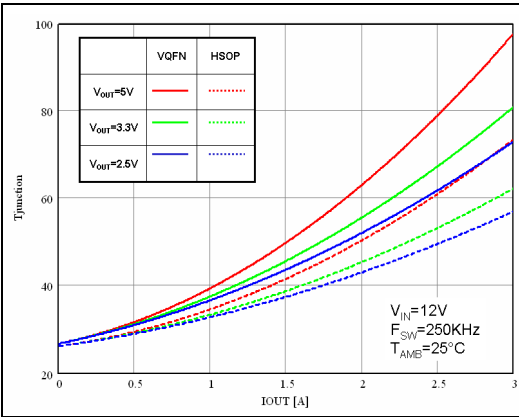
Figure 23. Junction temperature vs output current V_{IN} = 12\text{ V}
