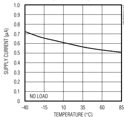
MAX5235 FULL POWER-DOWN SUPPLY CURRENT vs. TEMPERATURE
