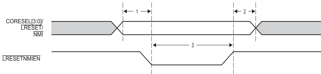
Figure 7-33 \overline{\text{NMI}} and Local Reset Timing
