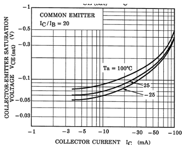
Fig. 10.20 RN2902FE V_{CE(sat)}-I_C
