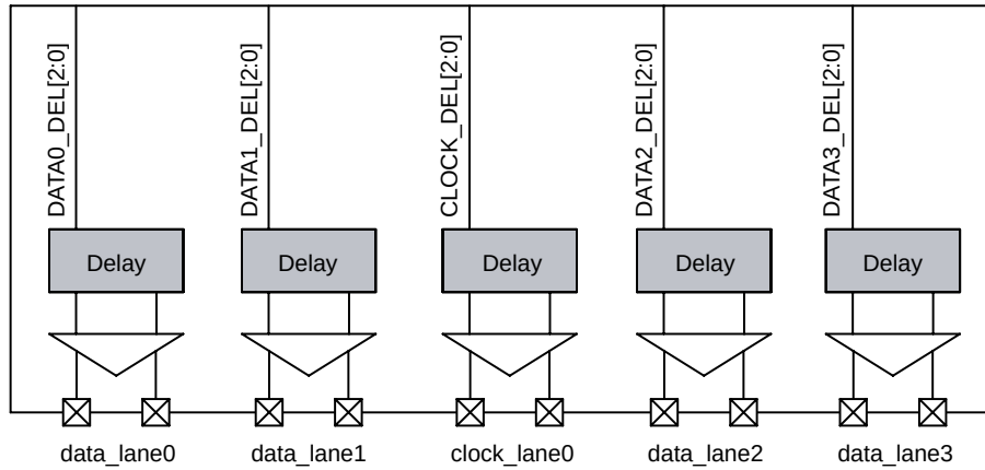
Figure 51. Block Diagram of DLL Timing Adjustment
