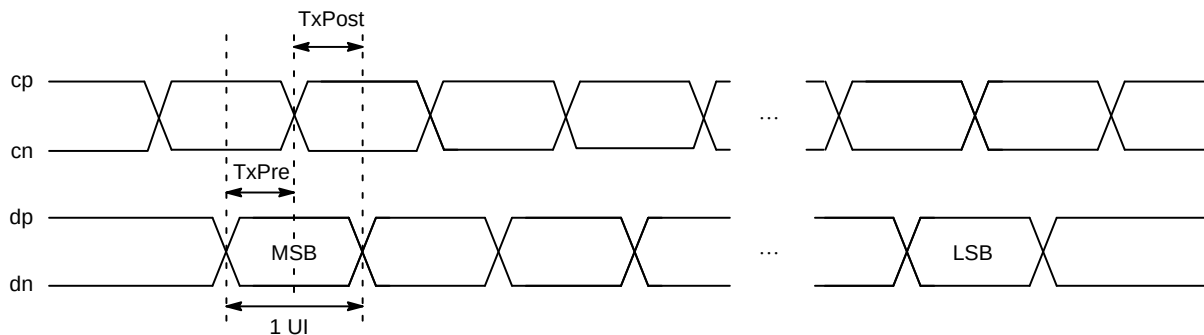
Figure 50. Timing Diagram
