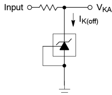
Figure 3: Off-State Current
