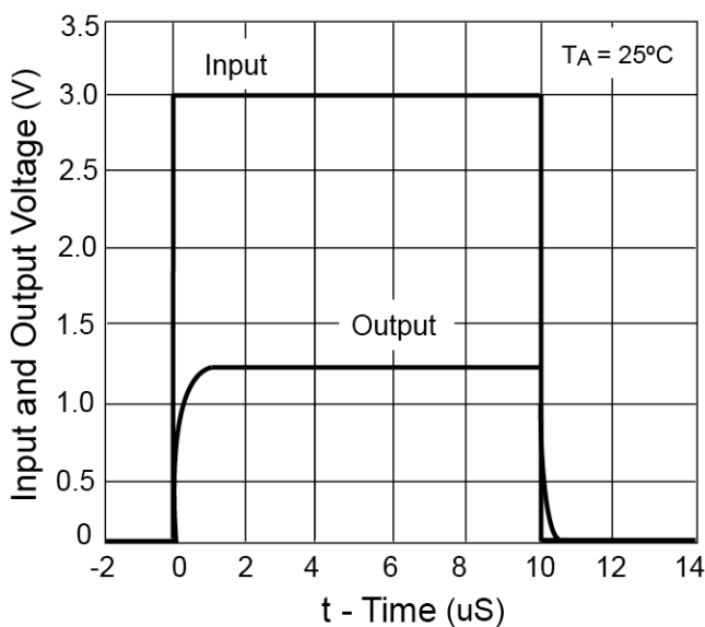
Figure 18: Pulse Response
