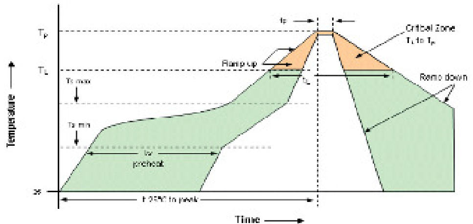
Solderprofile:
