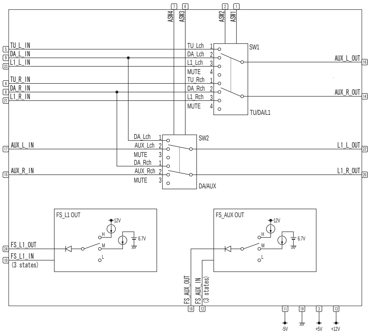
Fig.1 Block Diagram
