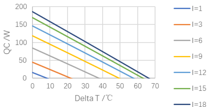
Performance Curves at T_h=27^\circ\text{C}
