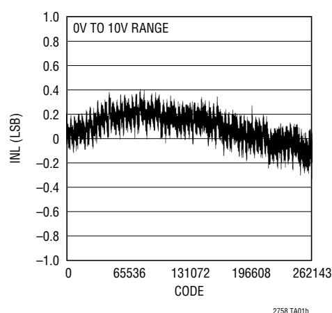
LTC2758 Integral Nonlinearity
