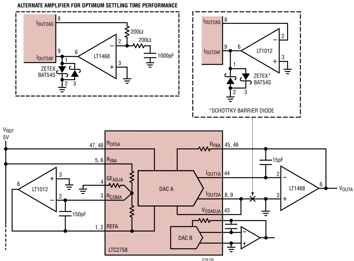
Figure 4. Optional Circuits for Driving I OUT2 from GND with a Force/Sense Amplifier
