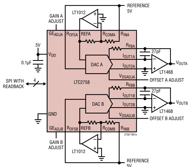
Dual 18-Bit V_{OUT} DAC with Software-Selectable Ranges
