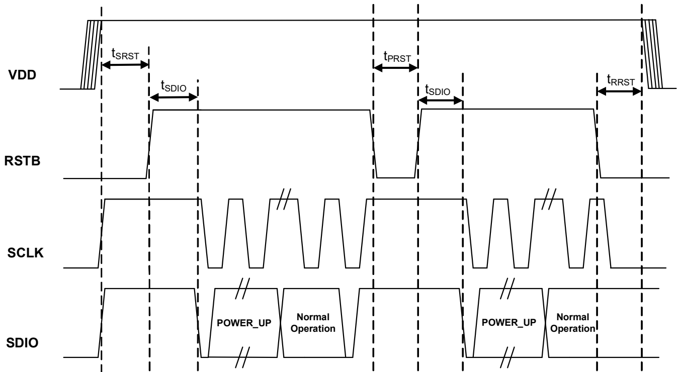
Figure 1. Reset Timing
