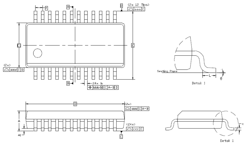
Figure 6. 24-Pin SSOP
