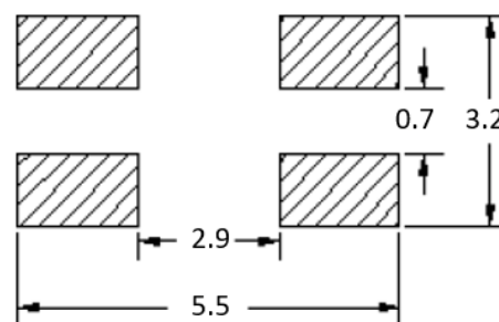
Recommended Layout
