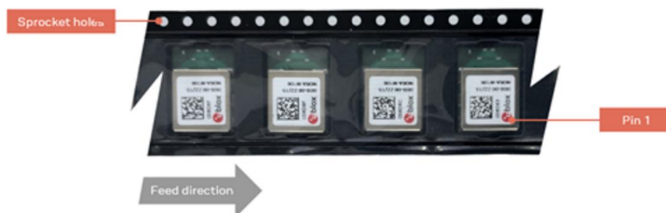
Figure 8: NORA-W406 module on tape orientation
