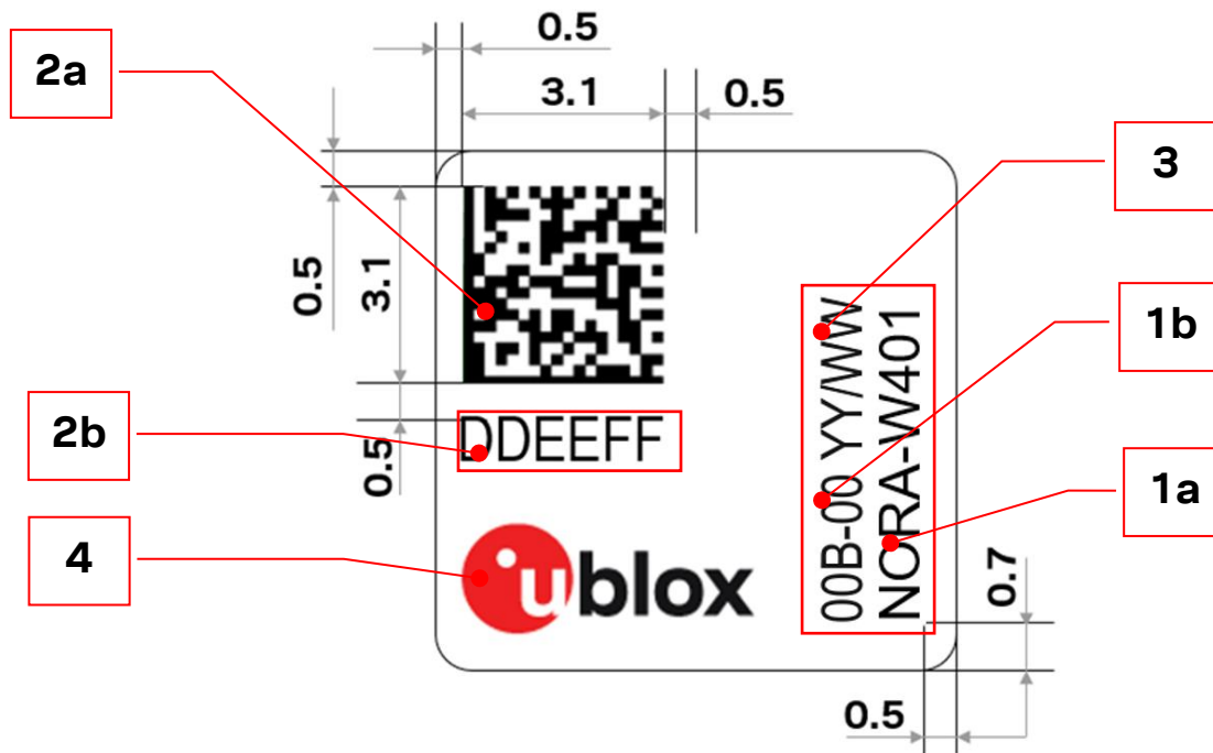
Figure 10: Location of product type number on the NORA-W40 series module label
