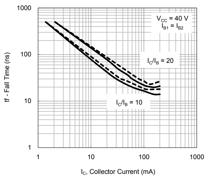
Fig.4 Fall Time
