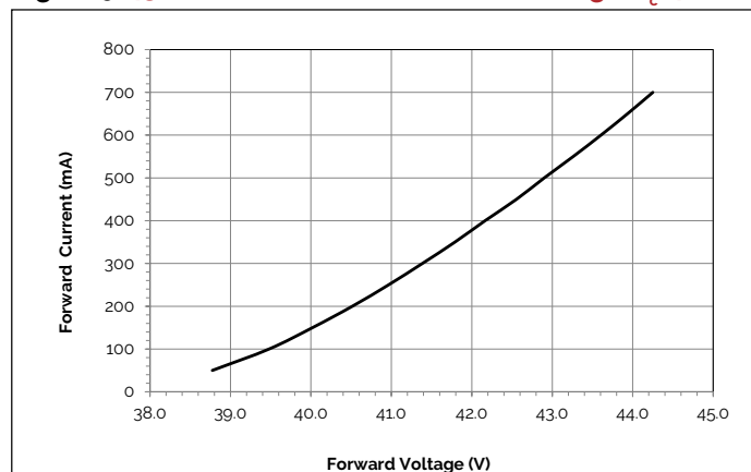
Figure 9: 43" Module Current vs. Forward Voltage, T_c=40^\circ\text{C}
