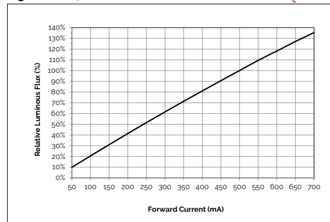
Figure 10: 43" Module Relative Flux vs. Current, T_c=40^\circ\text{C}
