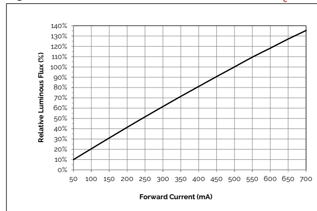
Figure 8: 21.8" Module Relative Flux vs. Current, T_c=40^\circ\text{C}
