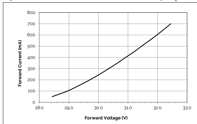
Figure 7: 21.8" Module Current vs. Forward Voltage, T_c=40^\circ\text{C}
