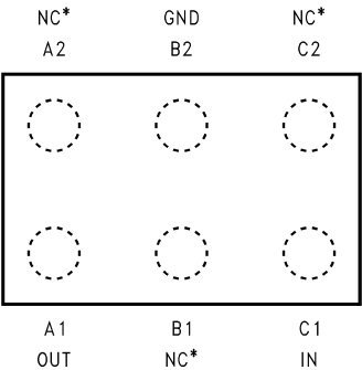
Figure 6. 6-Bump DSBGA Top View (Bump Side Down)
