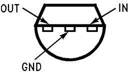
Figure 5. TO-92 Plastic Package Bottom View
