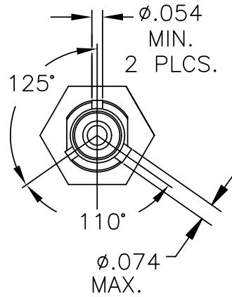
FIGURE 6 JACK INTERFACE "C"
