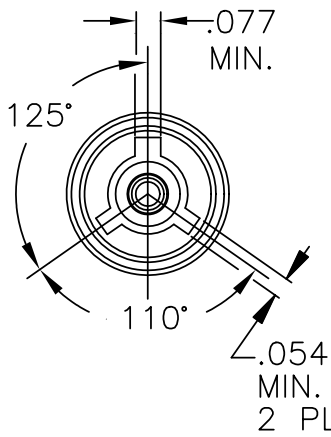
FIGURE 1 PLUG INTERFACE "A"
