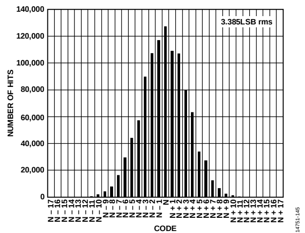
Figure 21. Input-Referred Noise Histogram, 2.5 V p-p FS
