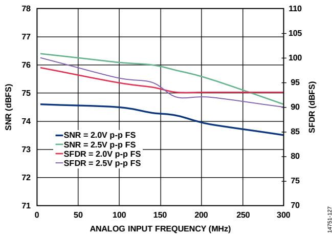
Figure 12. SNR/SFDR vs. f_{\text{IN}} , 2.0/2.5 V p-p FS
