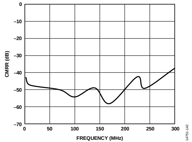
Figure 19. Common-Mode Rejection Ratio (CMRR)
