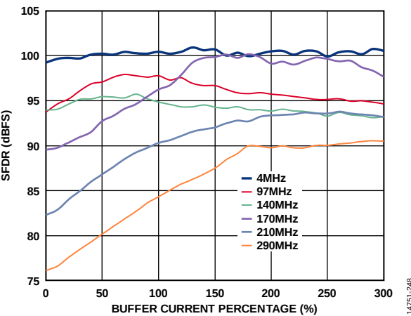
Figure 23. SFDR Performance vs. Buffer Current Percentage Over Analog Input Frequency
