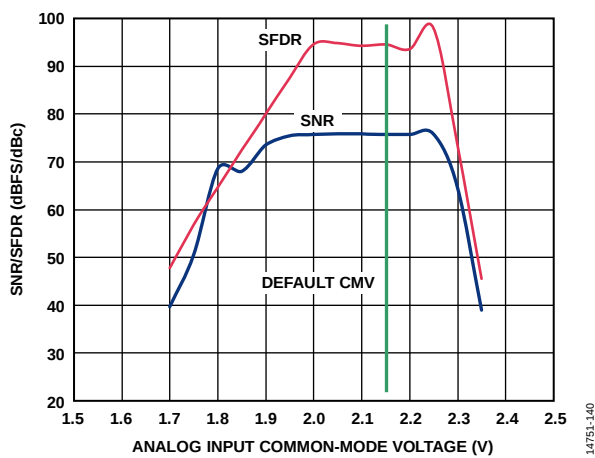
Figure 18. SNR/SFDR vs. Analog Input Common-Mode Voltage, A_{IN} = 100 MHz, 2.5 V p-p FS
