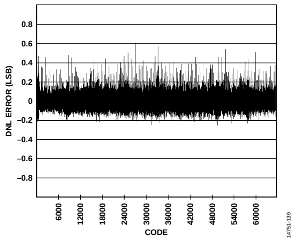
Figure 17. DNL, f_{IN} = 4.3 MHz, 2.5 V p-p FS
