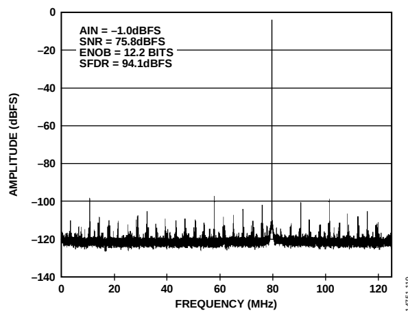
Figure 7. Single-Tone FFT with f_{IN} = 170.3 MHz, 2.5 V p-p FS
