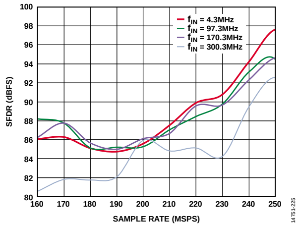
Figure 11. SFDR vs. f_{\text{SAMPLE}} , 2.5 V p-p FS
