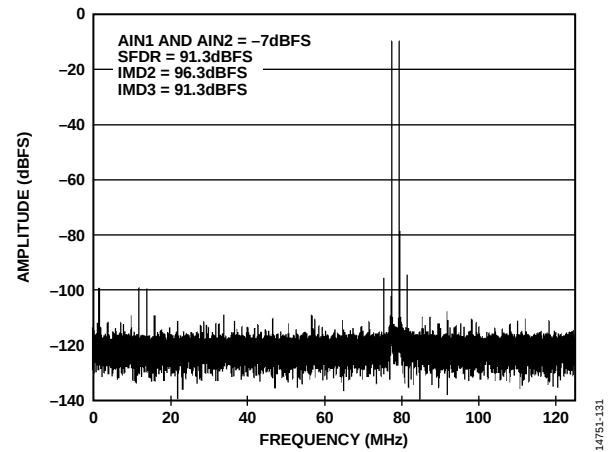
Figure 14. Two-Tone FFT with f_{\text{IN1}} = 170 MHz and f_{\text{IN2}} = 172 MHz, 2.5 V p-p FS
