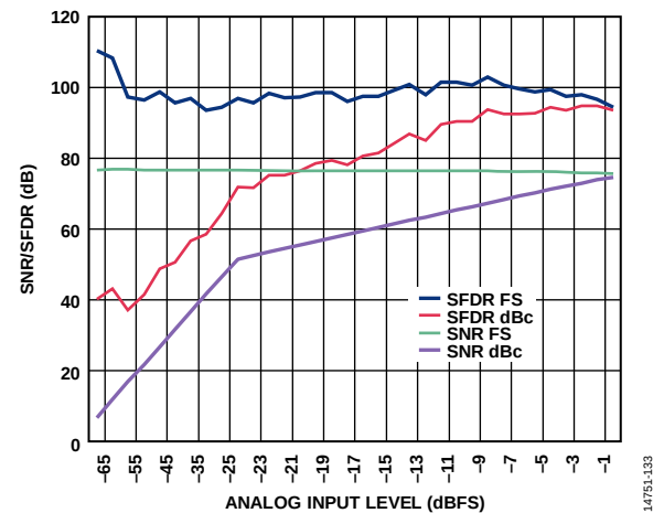
Figure 15. SNR/SFDR vs. Analog Input Level, f_{\text{IN}} = 97.3 MHz, 2.5 V p-p FS
