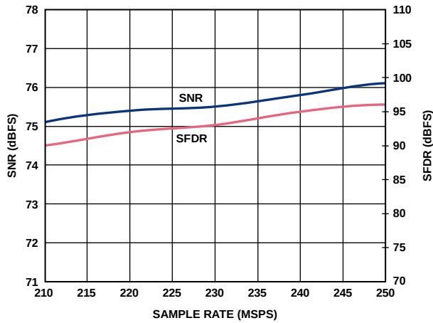
Figure 10. SNR/SFDR vs. f_{\text{SAMPLE}} , f_{\text{IN}} = 97.3 MHz, 2.5 V p-p FS
