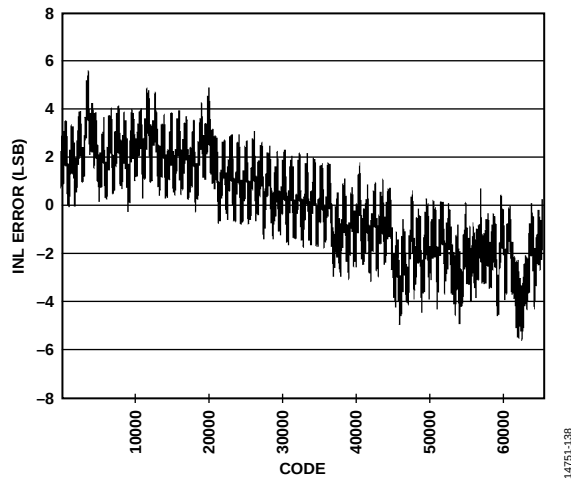
Figure 16. INL, f_{IN} = 4.3 MHz, 2.5 V p-p FS
