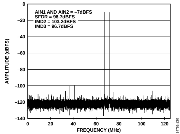
Figure 13. Two-Tone FFT with f_{\text{IN1}} = 70 MHz and f_{\text{IN2}} = 72 MHz, 2.5 V p-p FS
