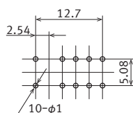
Recommended PC board pattern ( BOTTOM VIEW )
