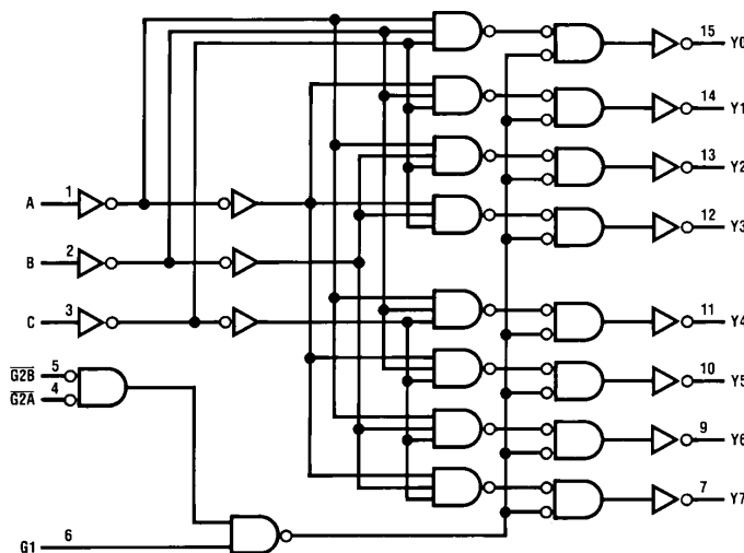
Figure 1. Logic Diagram
