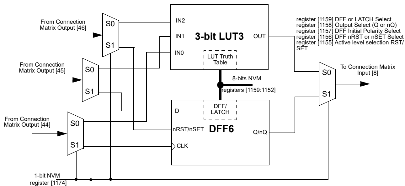
Figure 26: 3-bit LUT3 or DFF6
