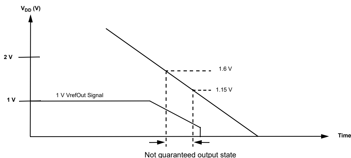
Figure 98: Power-Down
