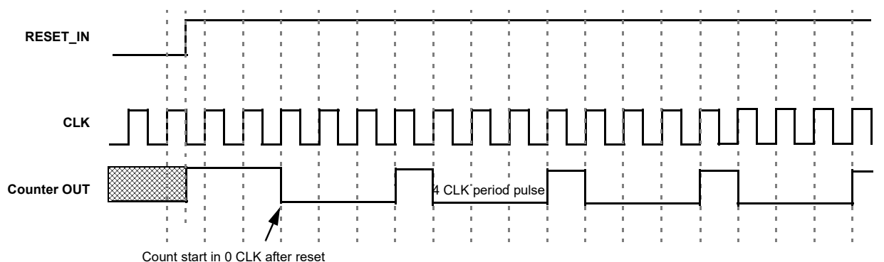
Figure 54: Counter Mode Timing Diagram with Two DFFs Synced Up
