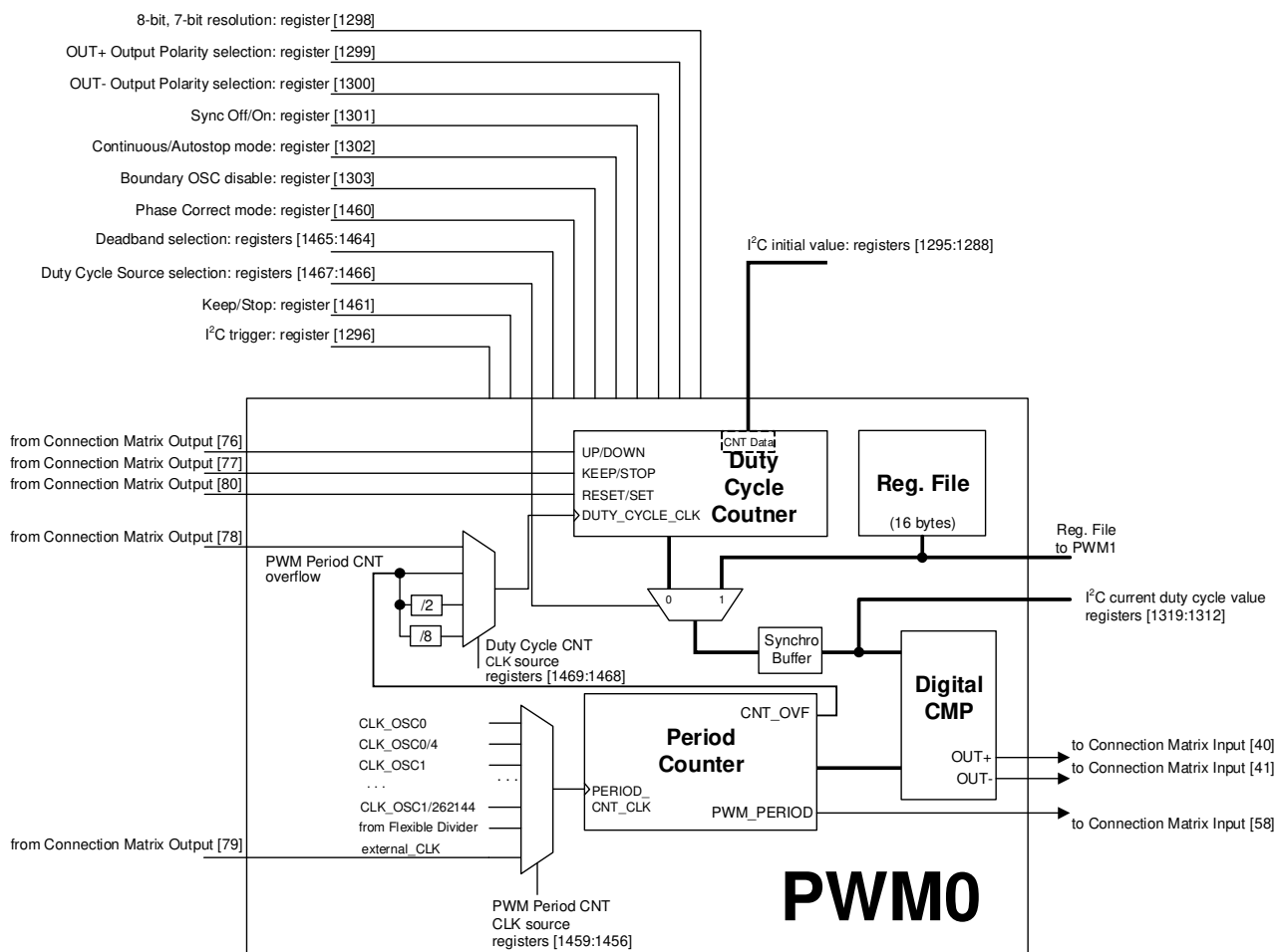
Figure 79: PWM0 Functional Diagram
