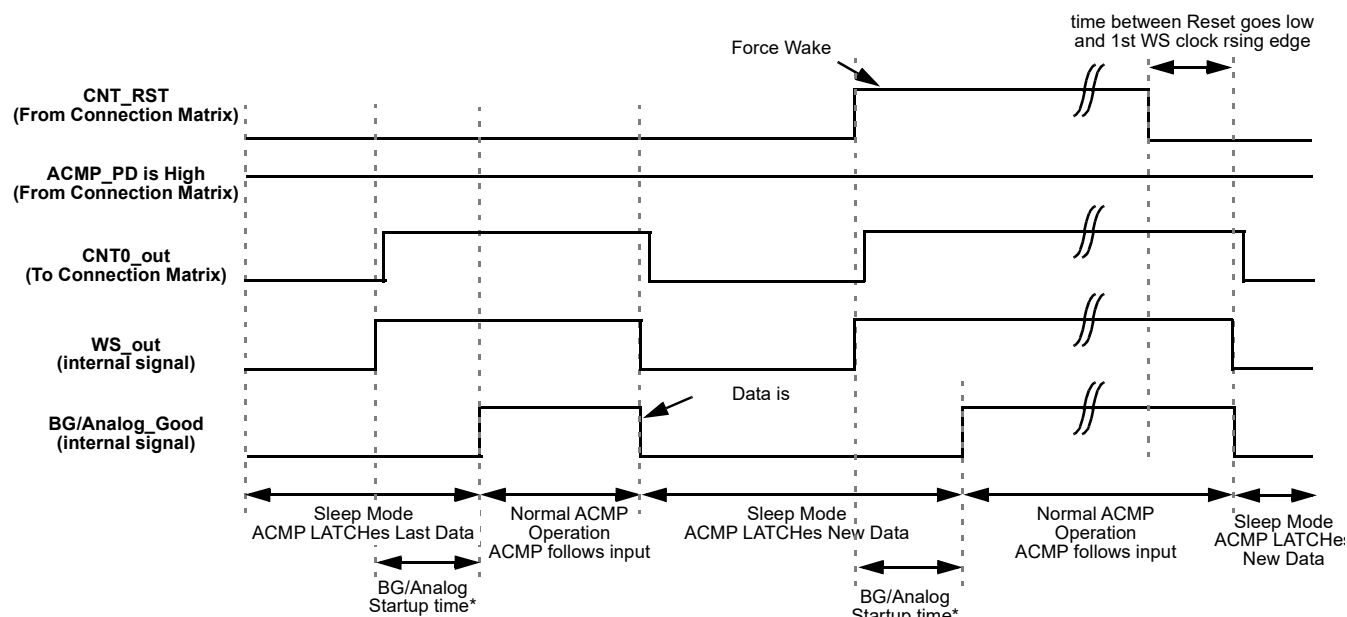
Figure 65: Wake/Sleep Timing Diagram, Normal Wake Mode, Counter Reset is Used
