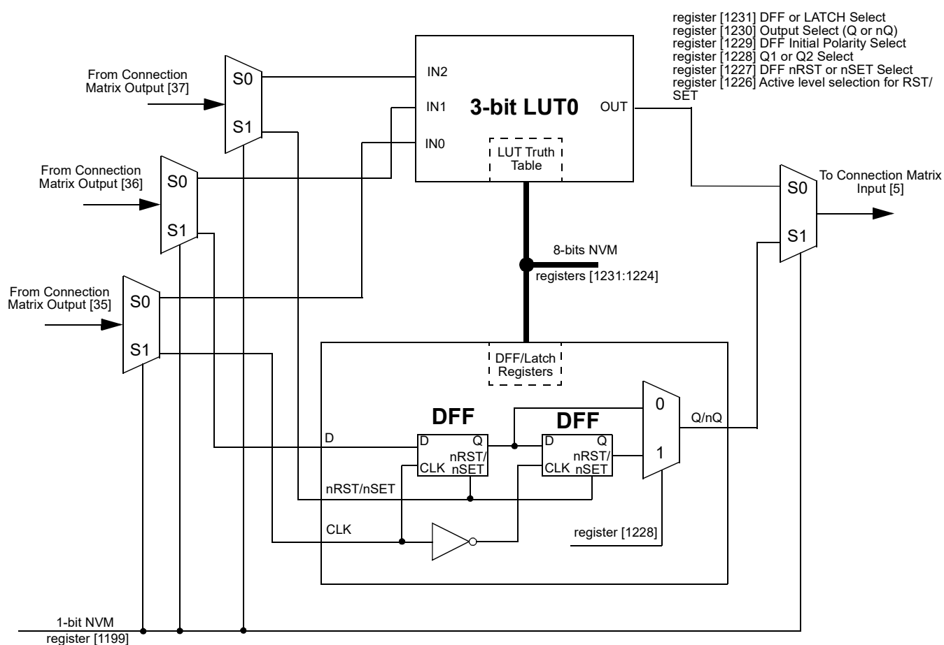
Figure 25: 3-bit LUT0 or DFF3
