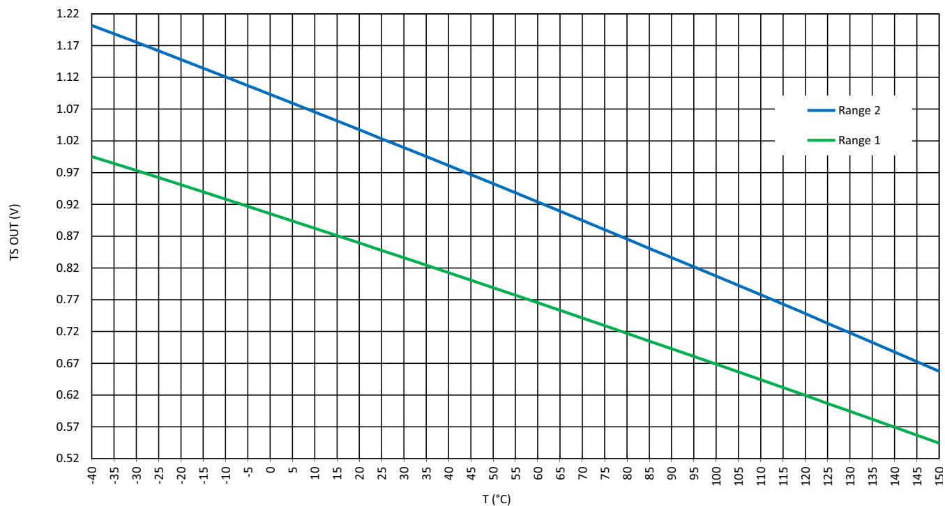
Figure 109: TS Output vs. Temperature, V_{DD} = 2.3\text{ V to }5.5\text{ V}
