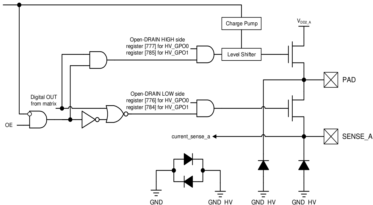
Figure 6: HV GPO Matrix OE IO Structure Diagram
