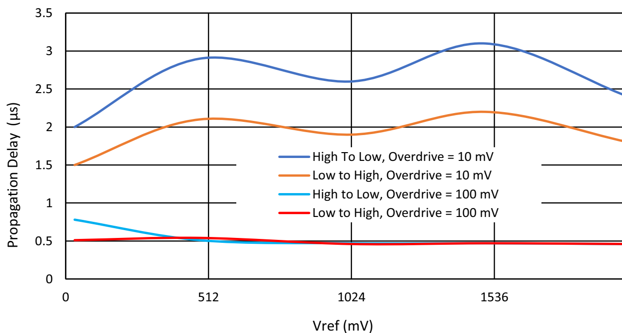
Figure 84: Typical Propagation Delay vs. Vref for ACMPxH at T = 25^\circ\text{C} , at V_{DD} = 2.3 \text{ V to } 5.5 \text{ V} , Gain = 1, Hysteresis = 0
