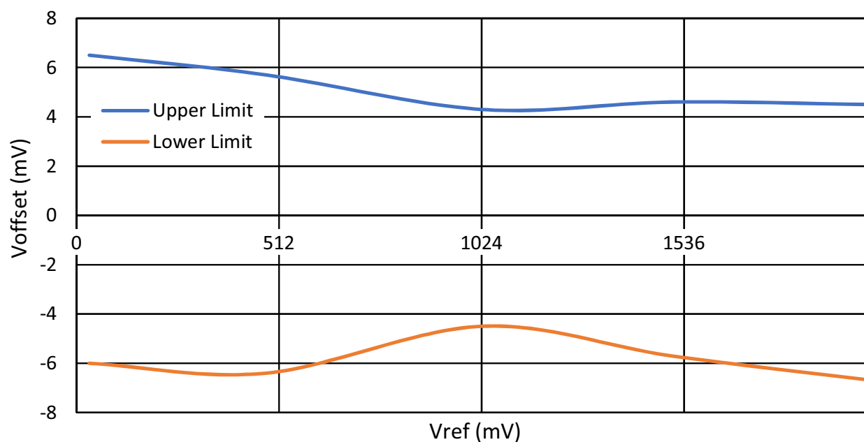
Figure 83: ACMPxH Input Offset Voltage vs. Vref at V_{DD} = 2.3 \text{ V to } 5.5 \text{ V} , T = -40^\circ\text{C to } 85^\circ\text{C} ,
