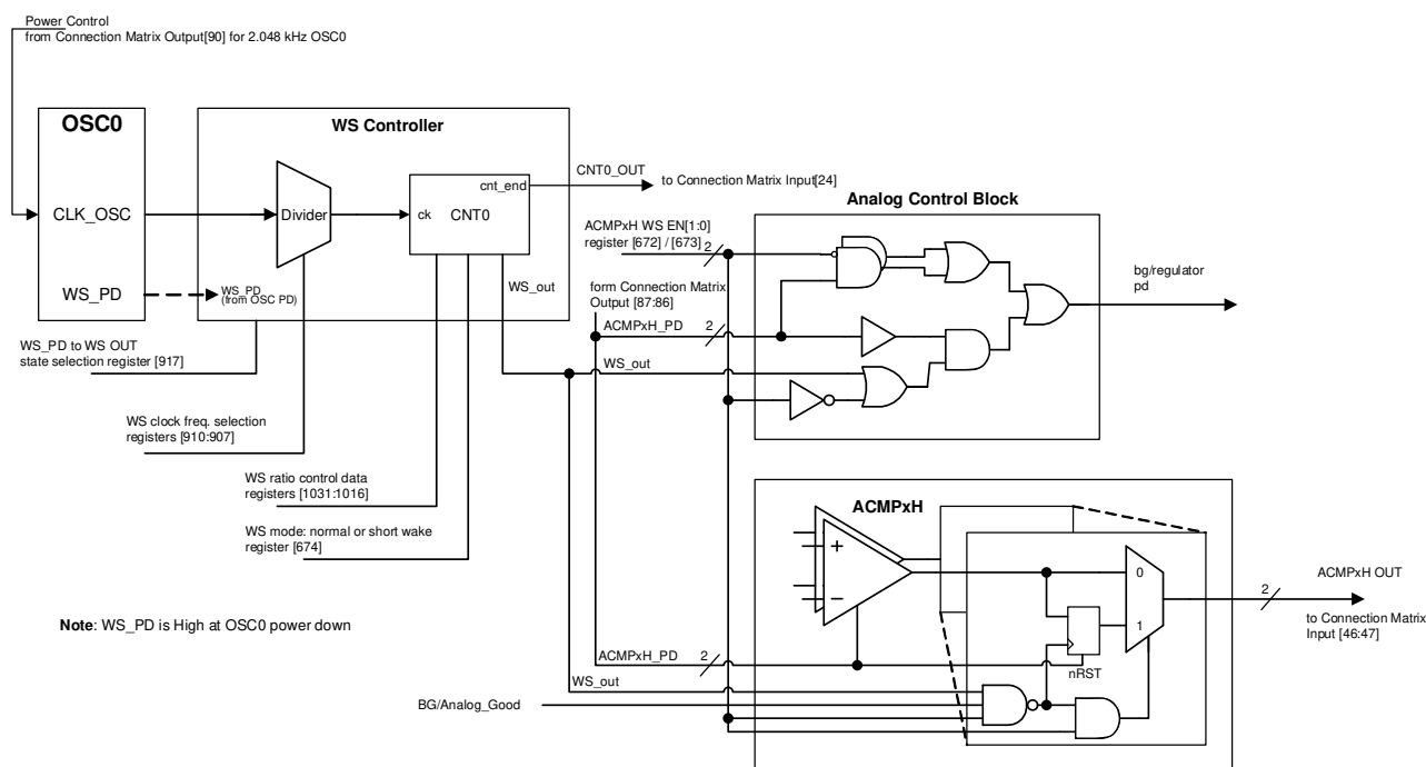
Figure 64: Wake/Sleep Controller
