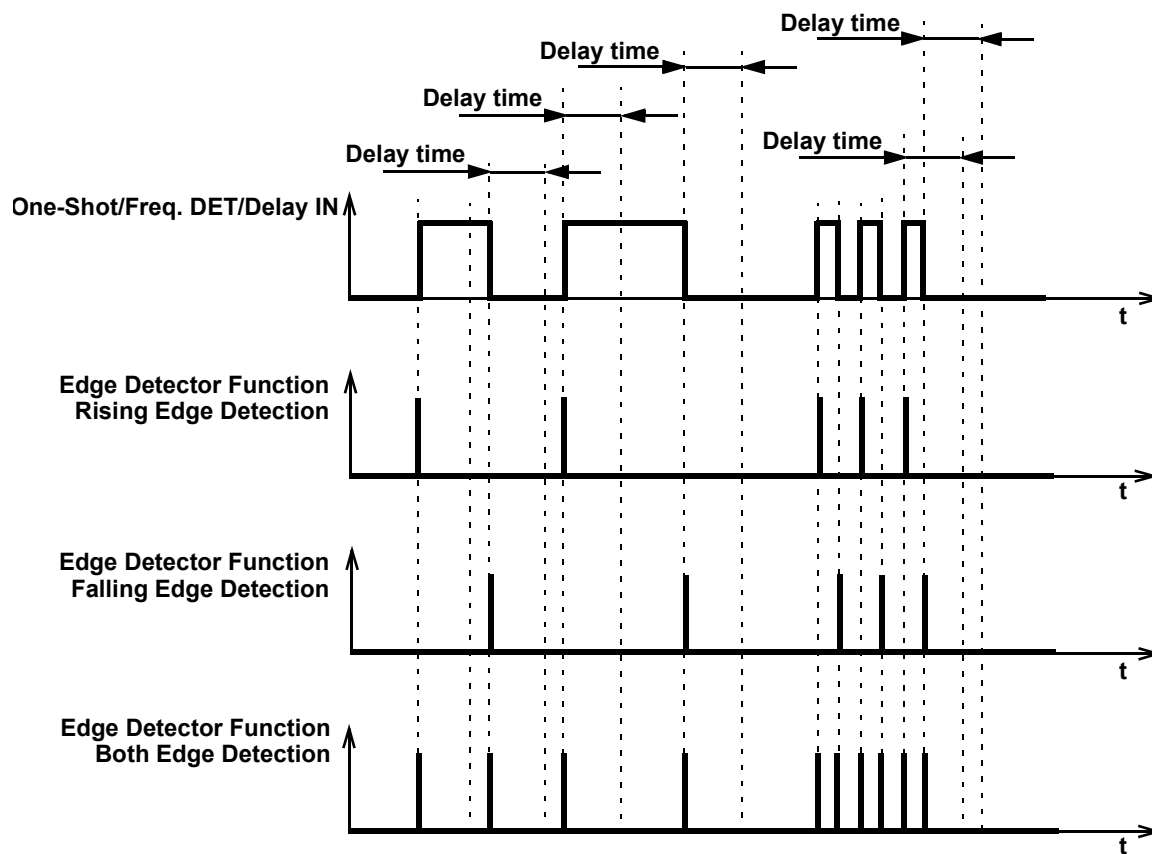
Figure 57: Edge Detection Mode Timing Diagram
