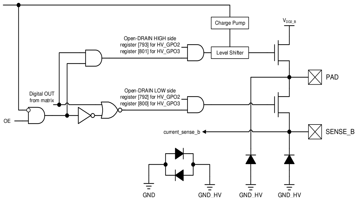
Figure 7: HV GPO Matrix OE IO Structure Diagram
