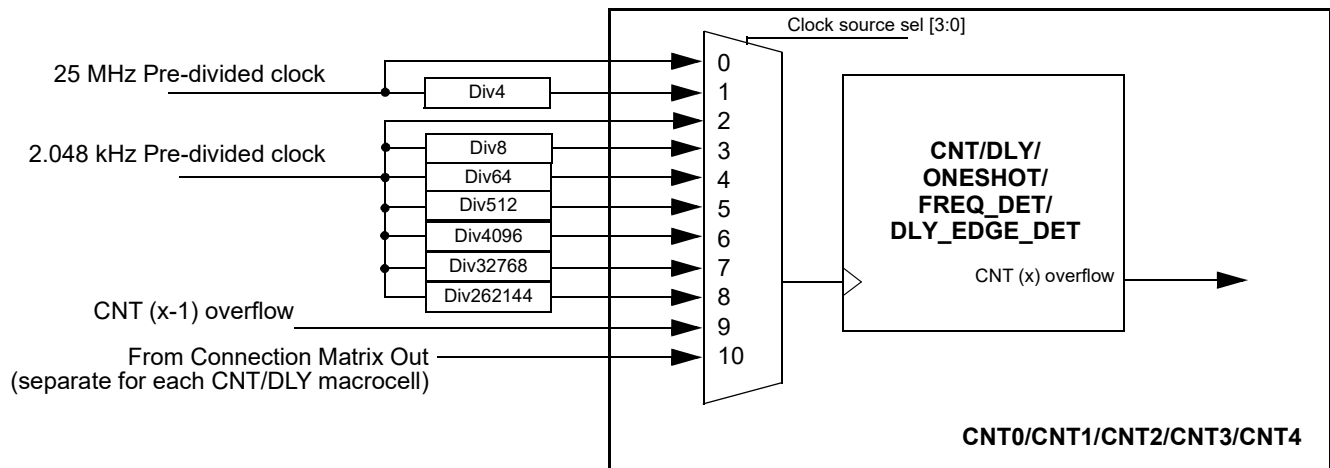
Figure 93: Clock Scheme
