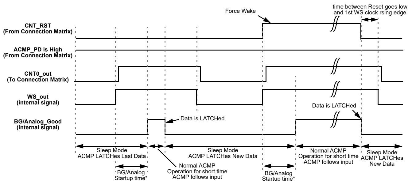
Figure 66: Wake/Sleep Timing Diagram, Short Wake Mode, Counter Reset is Used
