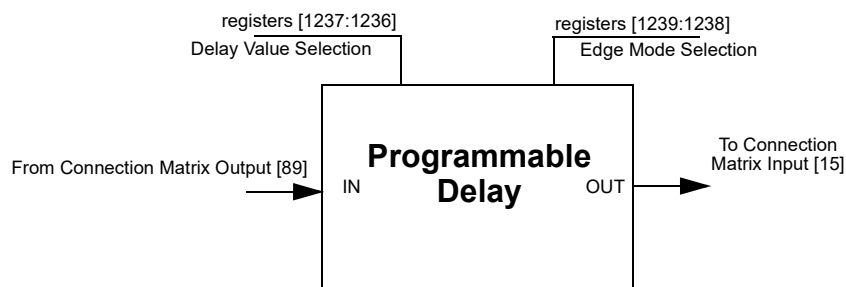
Figure 86: Programmable Delay
