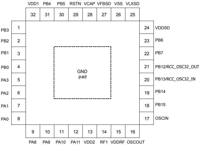
Figure 7. VFQFPN32 pinout
