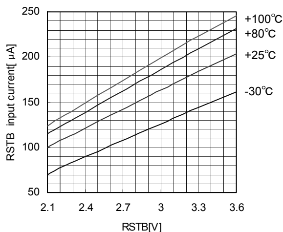
Fig.33 RSTB terminal voltage-RSTB inflow current (At the time of the current driver six lines use)
