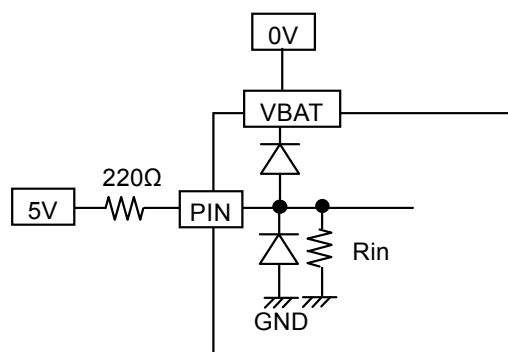
Fig.32 Voltage with a control sign higher than VBAT Example corresponding to application of conditions
