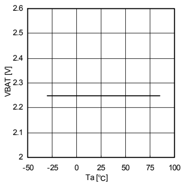
Fig.4 UVLO - Temperature
