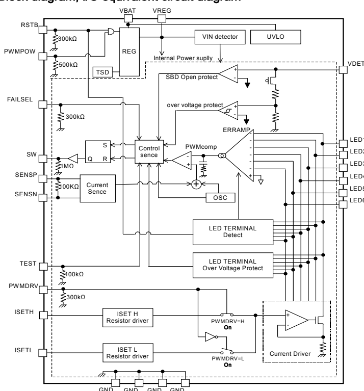
Fig.23 Block diagram
