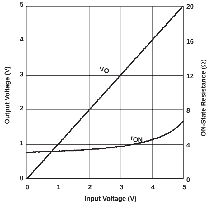
Figure 5. Output Voltage/ON-State Resistance vs Input Voltage
